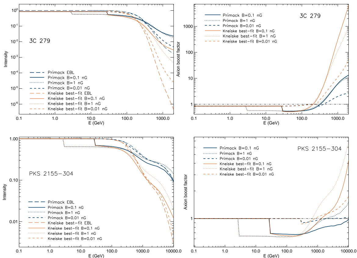
Figure 5.6 Same as in Figures 5.4 and 5.5 but for different values of IGMF. Upper panels: 3C 279 using those parameters listed in Table 5.2, only changing \mathbf{B} . Lower panels: Same exercise for PKS 2155-304, using the corresponding parameters that can be found in the same Table 5.2.
